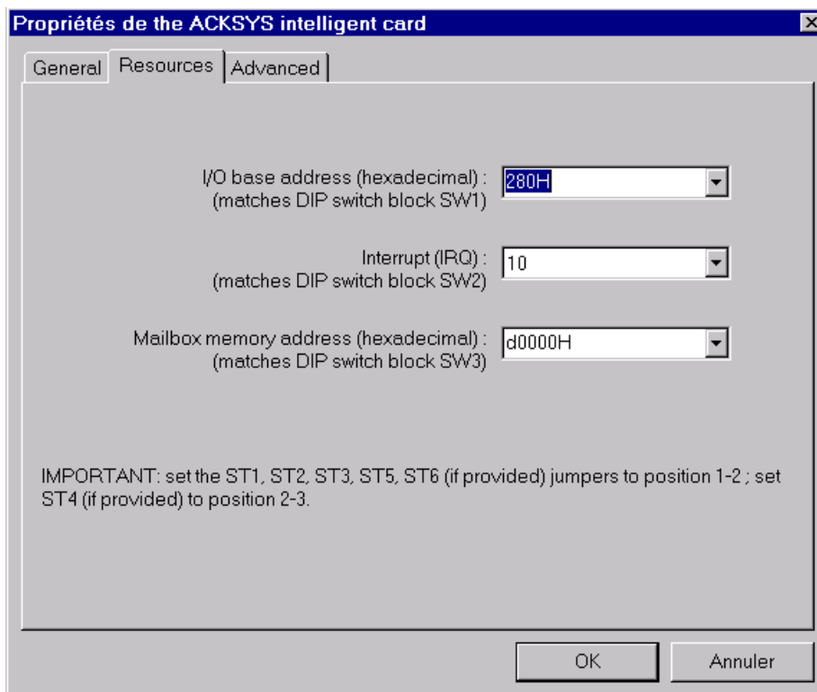
resources tab for ISA board
