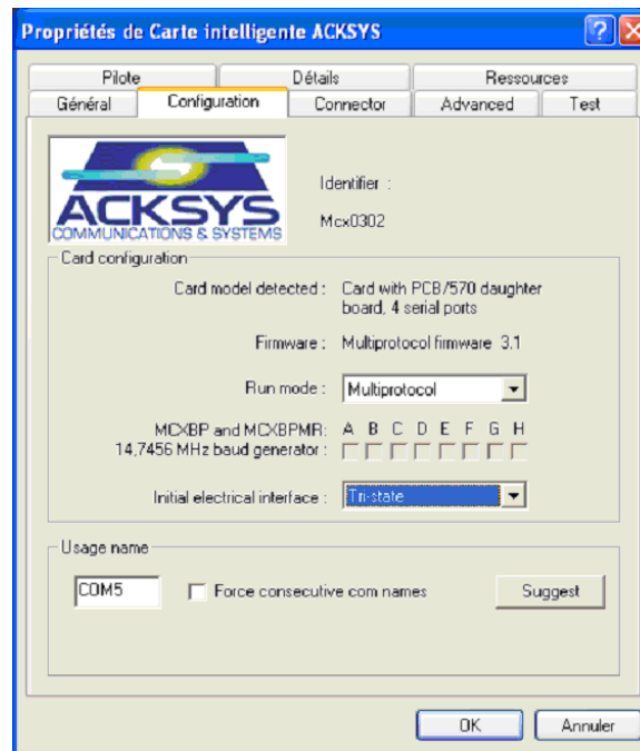
Board basic properties
