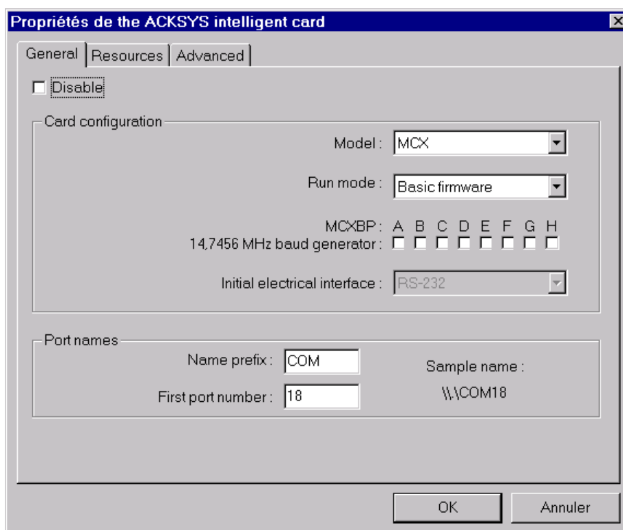
General properties of a board
